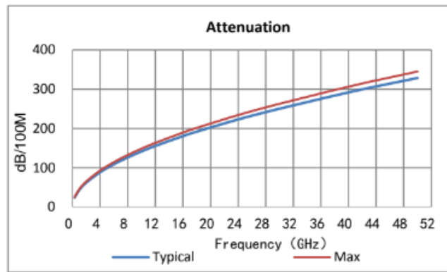
Attenuation (Typical@25°C&VSWR=1.0) &Power (VSWR=1.0;40°C;Sea Level)
